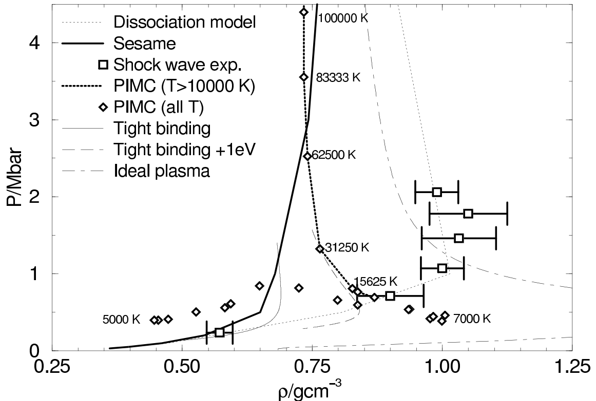
Figure 1. Comparison of Hugoniot from theory and experiment
