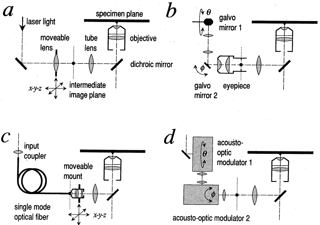
Figure 2 Four ways to scan the position of an optical trap in the specimen plane (see text). (a) Translating a moveable lens. (b) Rotating galvanometer mirrors. (c) Translating the end of an optical fiber. (d) Deflecting the beam with acousto-optic modulators (AOMs).
