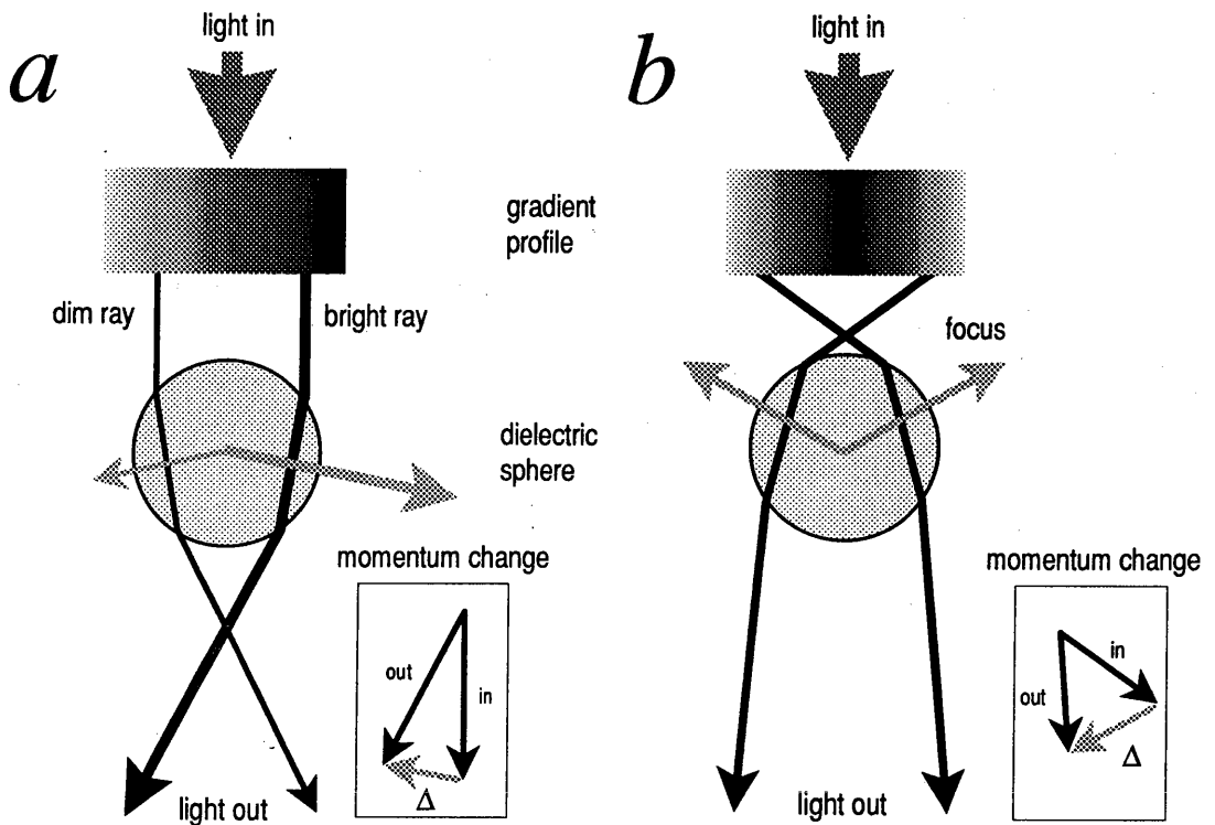
Figure 1 (a) A ray-optic picture of the gradient force. A parallel beam of light ( large gray arrow ) with a gradient in intensity ( shaded region ; the darker color indicates more light) shines through a transparent sphere with a higher refractive index than its background. The relative thickness of the two representative rays ( black arrows ) symbolizes intensity. The rays are refracted, giving rise to the reaction forces shown acting through the sphere's center ( gray arrows ). The brighter right ray conveys more force than the dimmer left ray: the sum of all rays in the beam tends to pull the sphere rightwards towards the light. ( Inset ) A vector diagram indicating the change of momentum for the right ray. The difference in momentum ( gray arrow ) produces an equal and opposite reaction in the sphere. (b) A single beam trap. Light ( large gray arrow ) is brought to a focus: its beam profile has an intensity gradient ( shaded region ). Two representative rays ( black arrows ) pass through a transparent sphere located beyond the focus. The rays are bent, and reaction forces ( gray arrows ) pull the sphere upwards, towards the focus. ( Inset ) A vector diagram indicating the change of momentum in the left ray. The difference in momentum ( gray arrow ) produces an equal and opposite reaction in the sphere.
